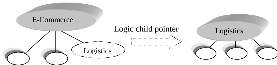
Fig. 3 : A logic child relationship diagram --- Using the relationships of E-commerce and Logistics as example
