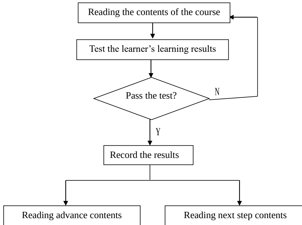
Fig. 7 : The flow chart of learner's learning monitoring mechanism
