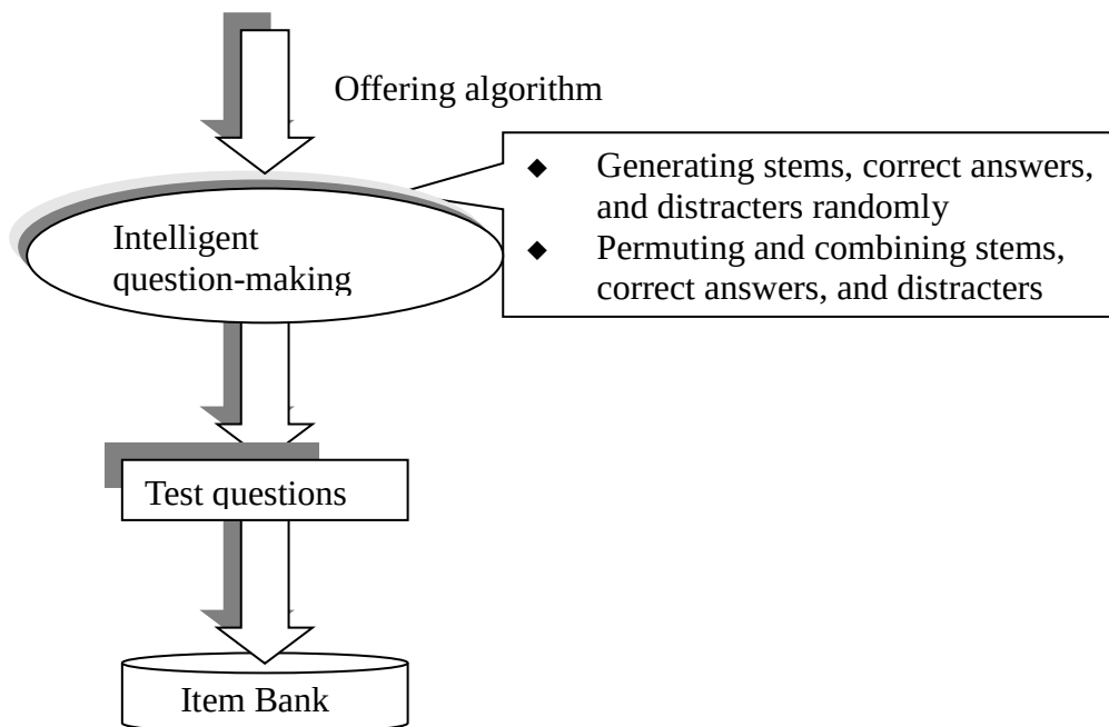
Fig.5 : The intelligent question-making mechanism I
