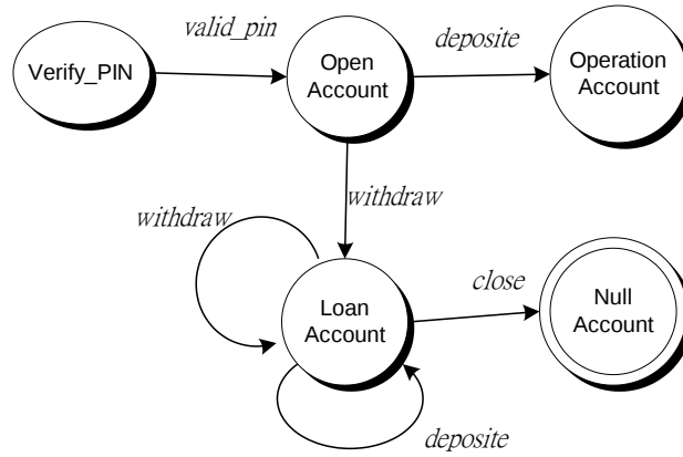
Figure 17. Illustration for (L_{test} \cap \overline{(L_{test} \cap L_{spec})}) \cup \overline{(L_{test} \cap (L_{test} \cap L_{spec}))}
