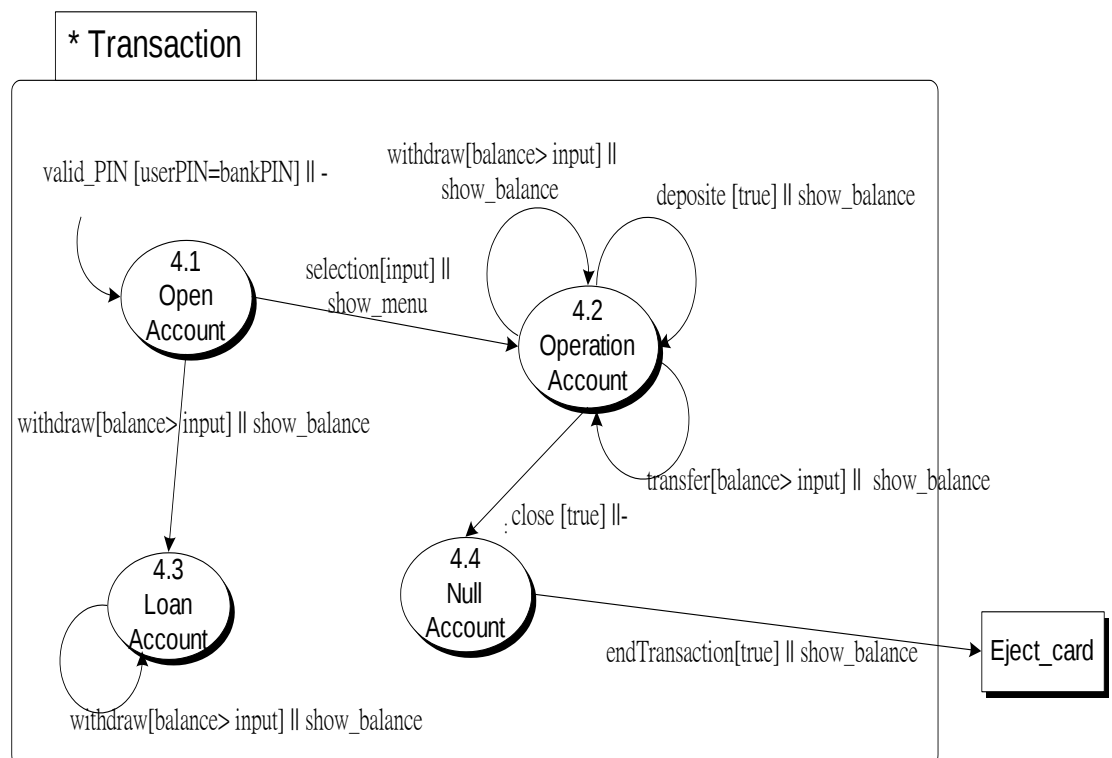
Figure 12. Transaction superstate in ATM
