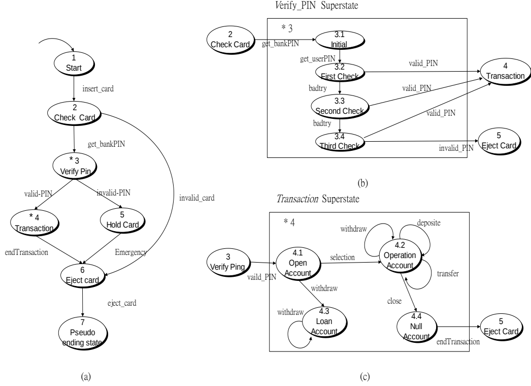
Figure 13. Convert the RSML specification to a corresponding finite automata
