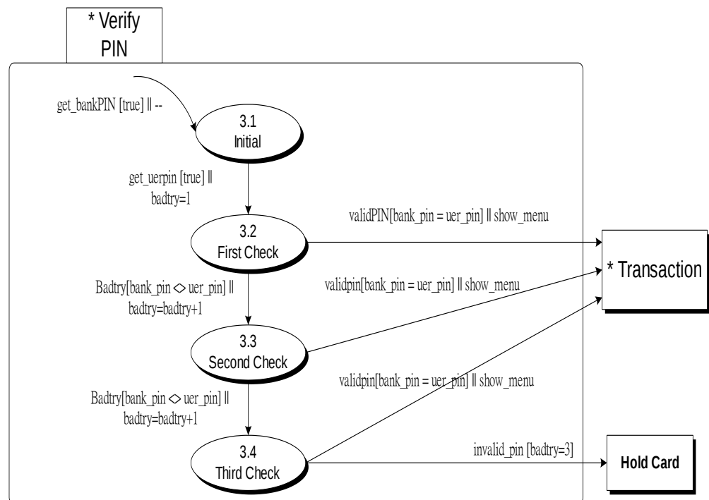
Figure 11. Verify PIN superstate in ATM
