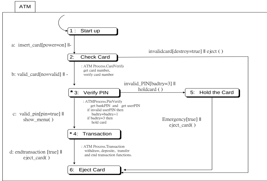
Figure 10. The RSML specification of ATM Transaction
