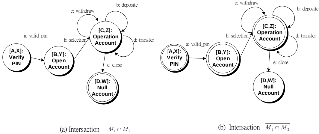
Figure 16. Illustration for L_{spec} \cap L_{test} and \overline{L_{spec} \cap L_{test}} respectively
