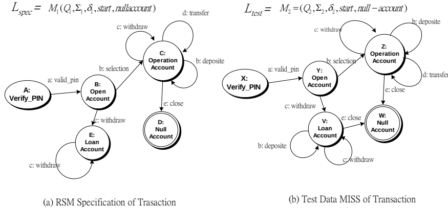
Figure 15. An illustration of the testing framework: using transaction state.
