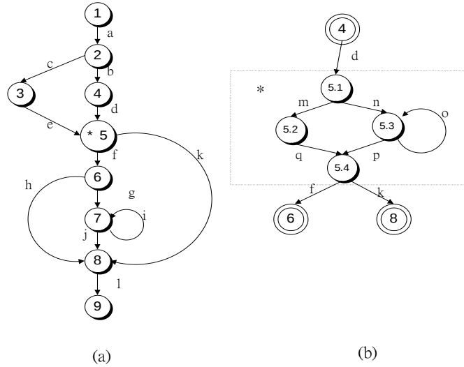
Figure 4: An example of STD
