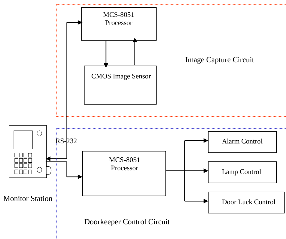
Figure 4: Block diagram of the doorkeeper system
