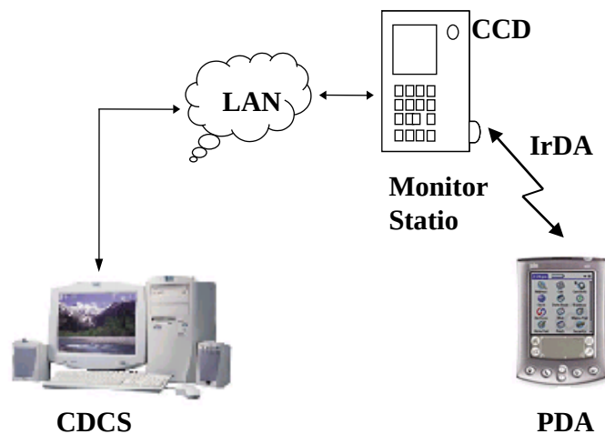
Figure 1: The architecture of doorkeeper system based on wireless IrDA interface
