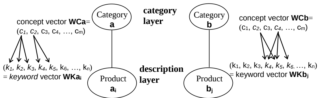
Figure 4: The product data architecture
