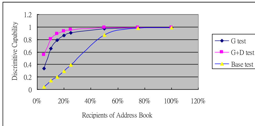
Figure 8 The discriminative capability from simulated behavior based on both analysis compared with base test
