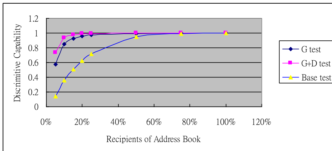
Fig. 9 Discriminative capability determined from simulated behavior based on 1823 mailers.
