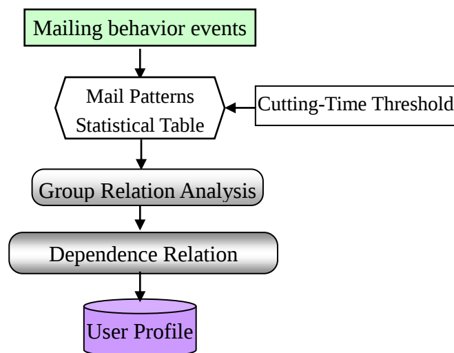
Figure 3 The flow of processing mailing behavior with table of mailing behavior statistics and the cutting-time
