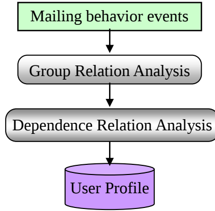
Figure 2 Flow for building a user profile
