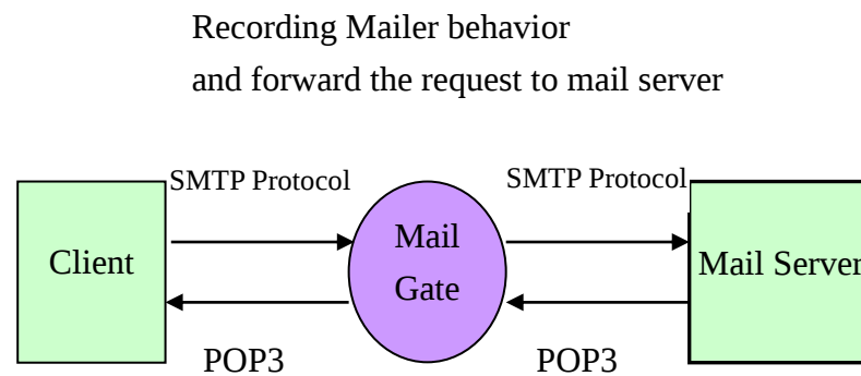
Figure 10 The architecture of the Mail Gate alarm system
