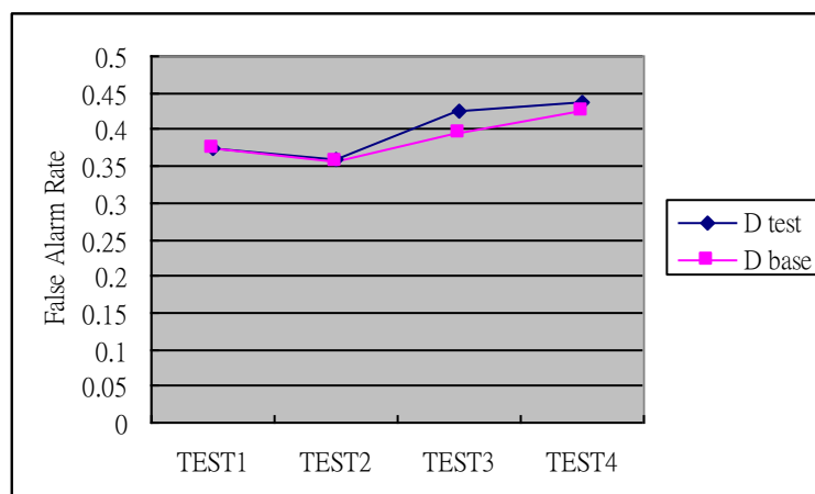
Figure 7 The average false alarm rates for the sliding window and the base data (only conditions for group and dependence analysis are shown, result of the group relation analysis is similar too)
