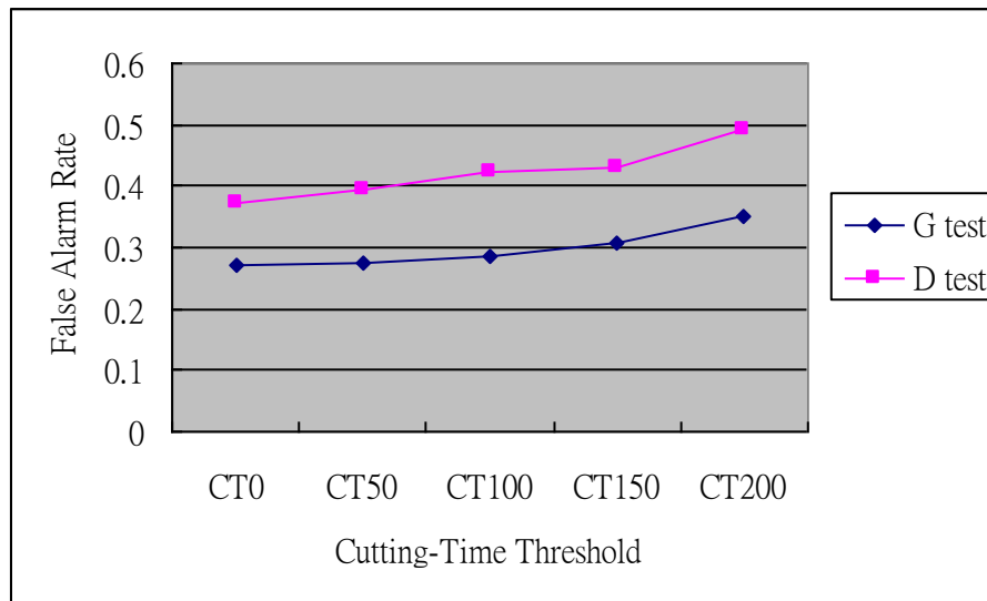
Figure 6 The average false alarm rate for different cutting-time thresholds
