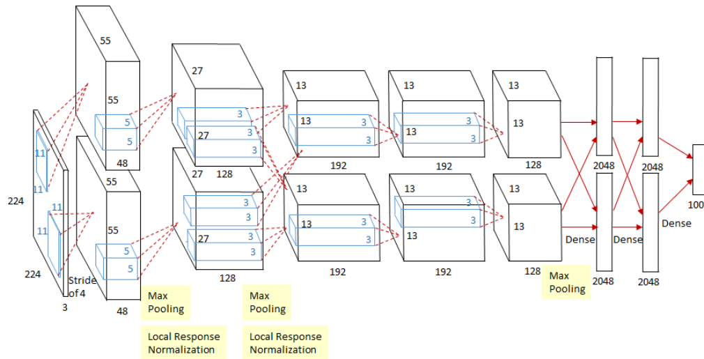
Figure 6: An illustration of the AlexNet architecture and running on two GPUs [23]
