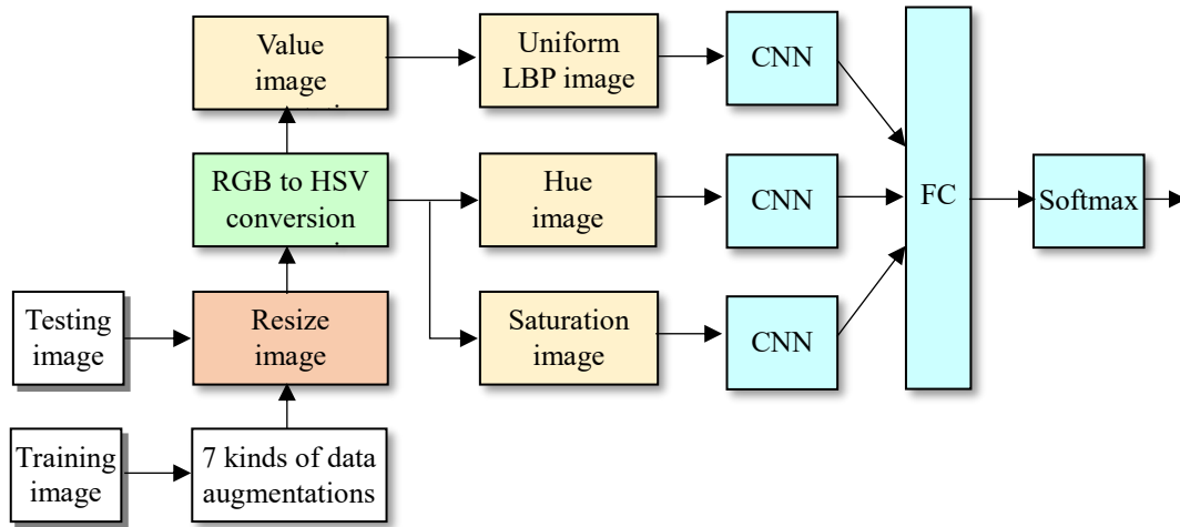
Figure 9: The architecture of the proposed Multi-channel CNN (MCCNN)
