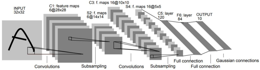
Figure 5: An illustration of the architecture of LeNet [22].
