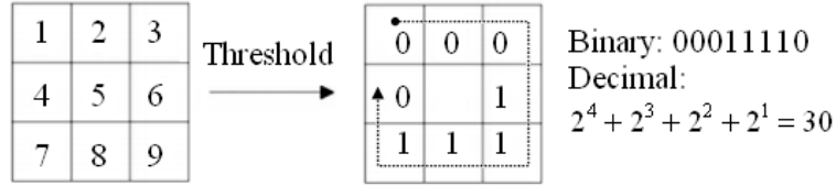
Figure 2: An example of the pattern and LBP
