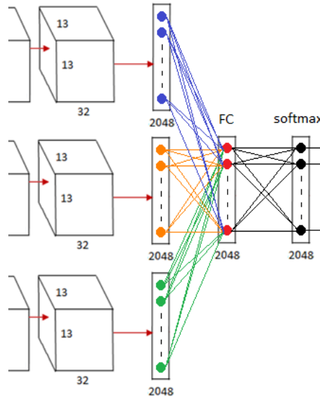
Figure 13: Overview of the fully connected (FC) layer
