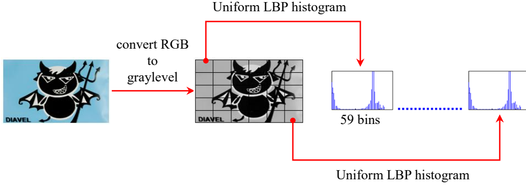
Figure 4: Uniform LBP based image description
