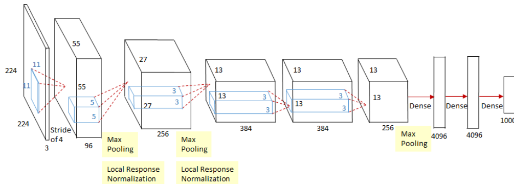
Figure 7: An illustration of the CaffeNet architecture and running on single GPU [24]
