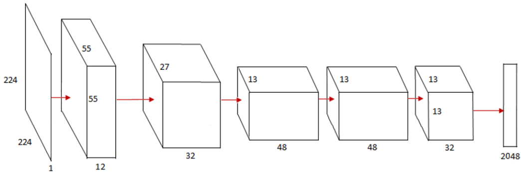
Figure 12: Overview of the proposed CNN
